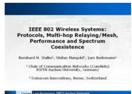
example screenshot 2
