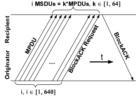
Fig. 2. Message Sequence Chart on the frame exchange procedure using BA. The reception of MSDUs may be interrupted at any time. Thus only after having received a BlockACK Request in the same or in a subsequent TXOP the receiver replies by a BlockACK frame.
