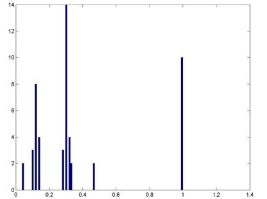
Fig. 6: Histogram of \varpi for L_{p2}
