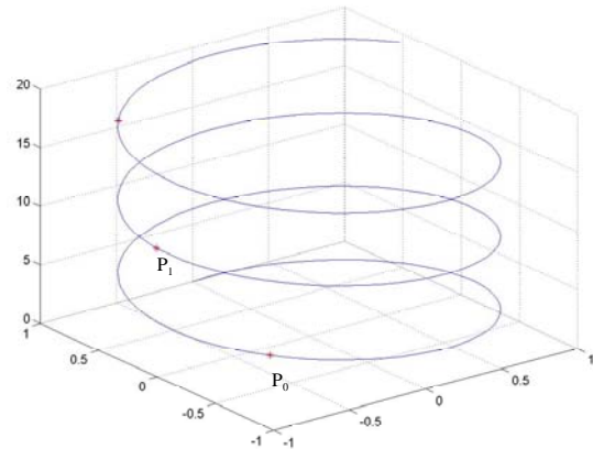
Fig. 2: A helix given by the Eq. (1), for \varpi = 1 .
