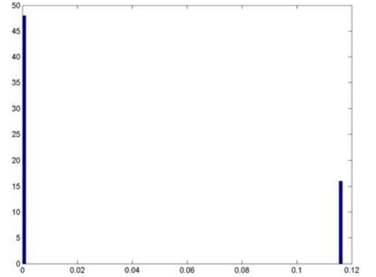
Fig. 5: Histogram of \varpi for L_{p1}
