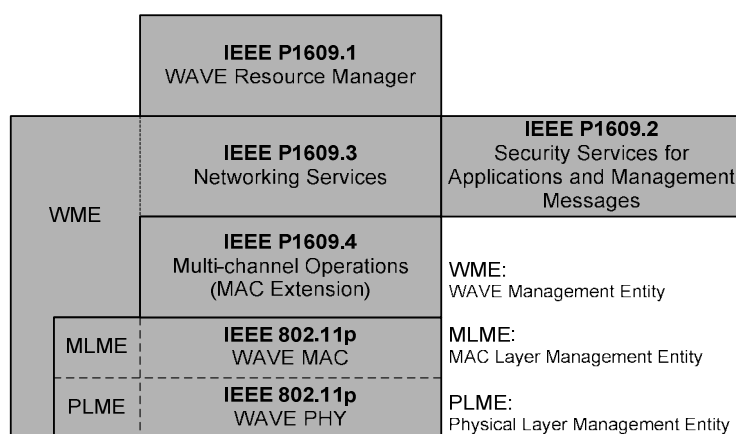
Figure 2. Protocol stack of WAVE system
