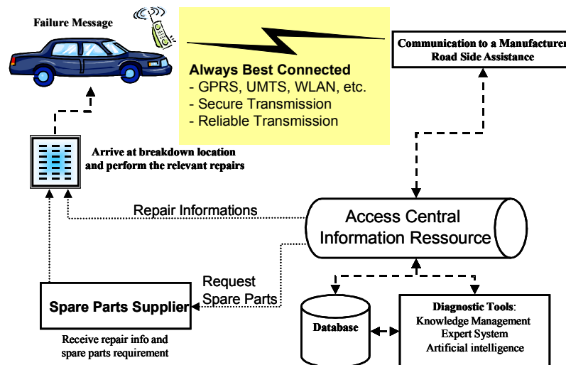
Figure 1. MYCAREVENT information flow
