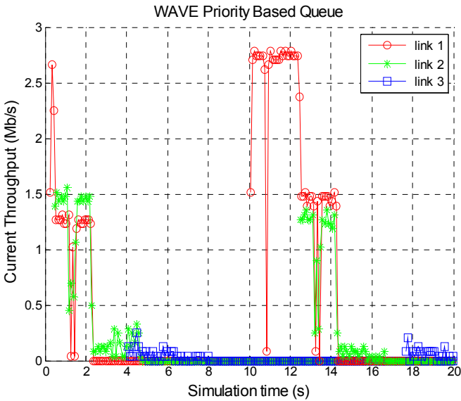
Figure 13. Instant throughput without link based MAC queue
